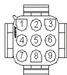
CHASSIS HARNESS CONNECTOR (C1) (MATING SIDE)
